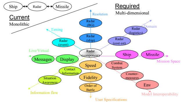
Figure 2: Complexity of Module Descriptors
